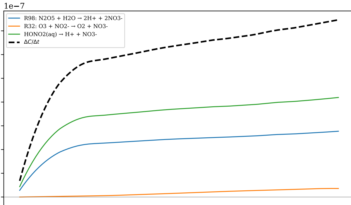
(a) \text{NO}_3^-
